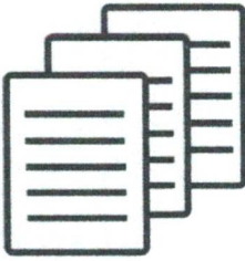
.rox file
